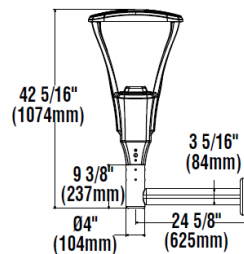
WM Wall Mount Bracket 1.5G rated Wall Mount Arm mounts to standard 4" steel J-Box (Supplied by others) and is provided with masonry anchors for extra support.
